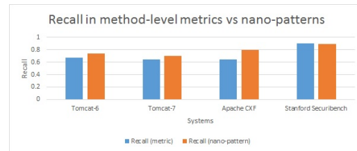
(b) Recall of nano-patterns and method-level metrics
