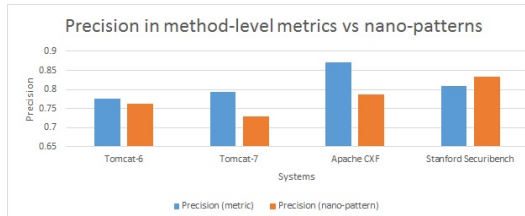
(a) Precision of nano-patterns and method-level metrics
