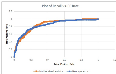
Fig. 7: ROC for nano-patterns and method-level metrics
